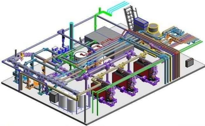
Chiller Management system
